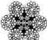
6 x 36 Warrington-Seale
