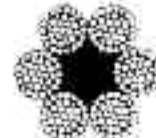
6 x 37* Warrington
